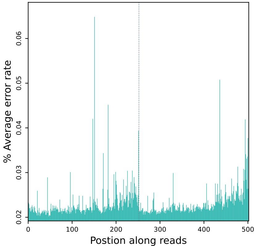
Error rate distribution along reads (R20209)
